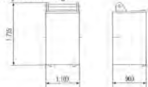
Carbody Counterweight
