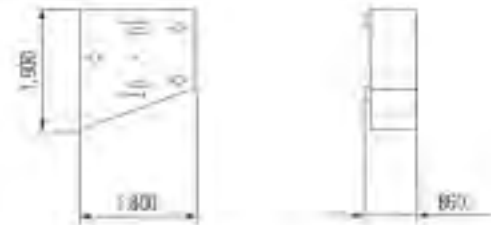
Counterweight
